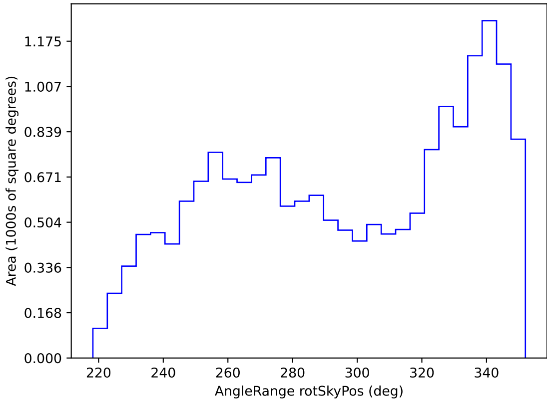
ddf_loaded_fl2_v3.4_10yrs WFD all bands: AngleRange rotSkyPos
