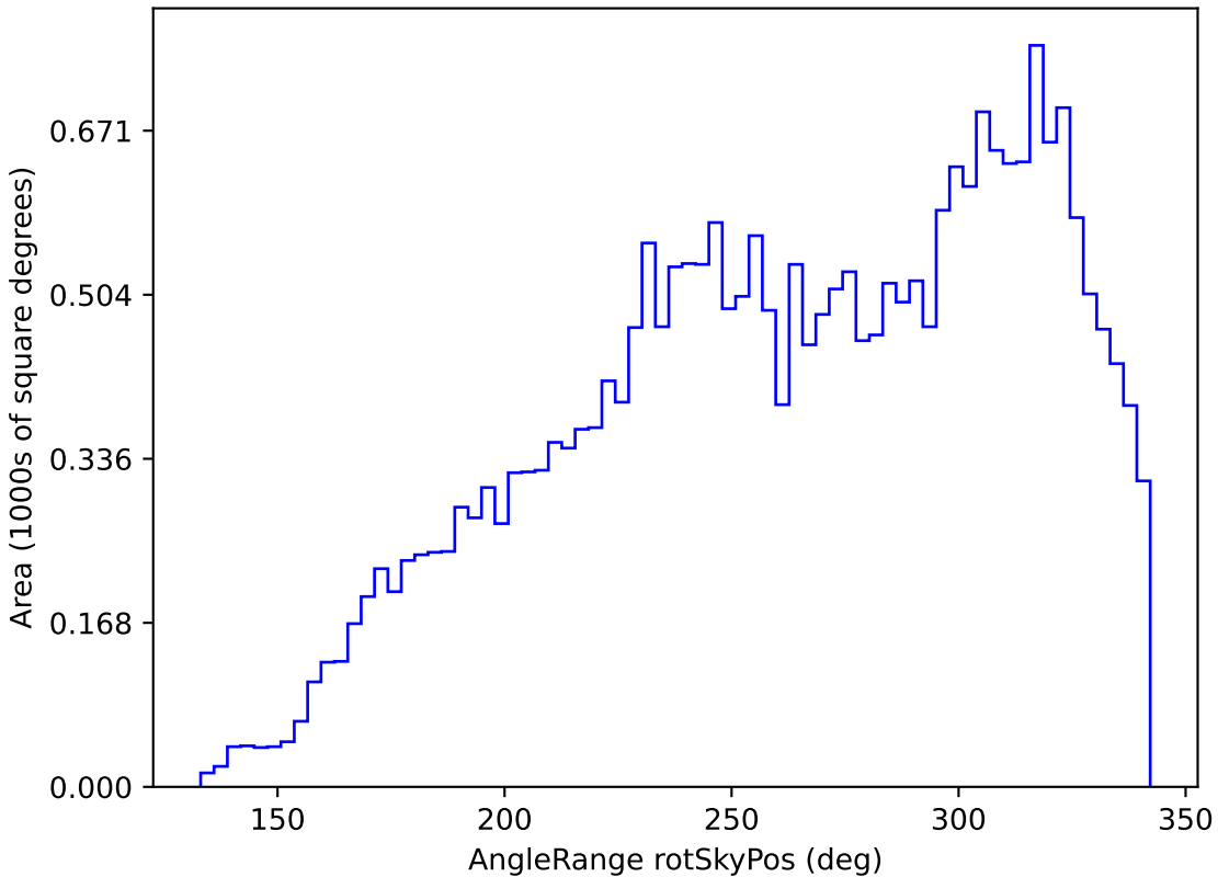
ddf_loaded_fl2_v3.4_10yrs All sky z band: AngleRange rotSkyPos
