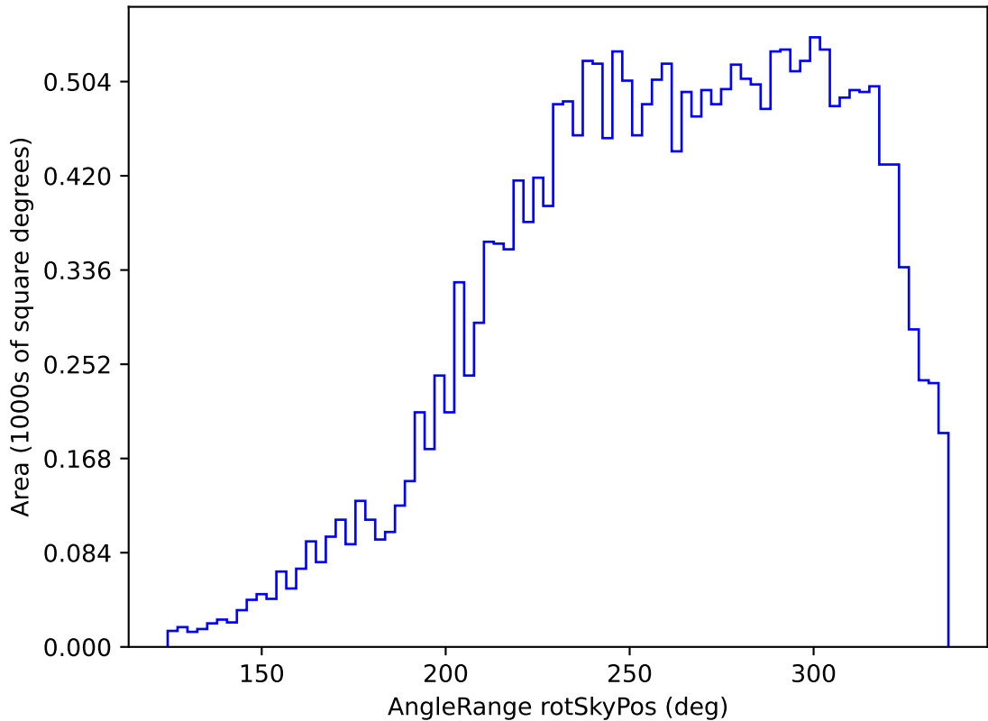
ddf_loaded_fl2_v3.4_10yrs All sky y band: AngleRange rotSkyPos
