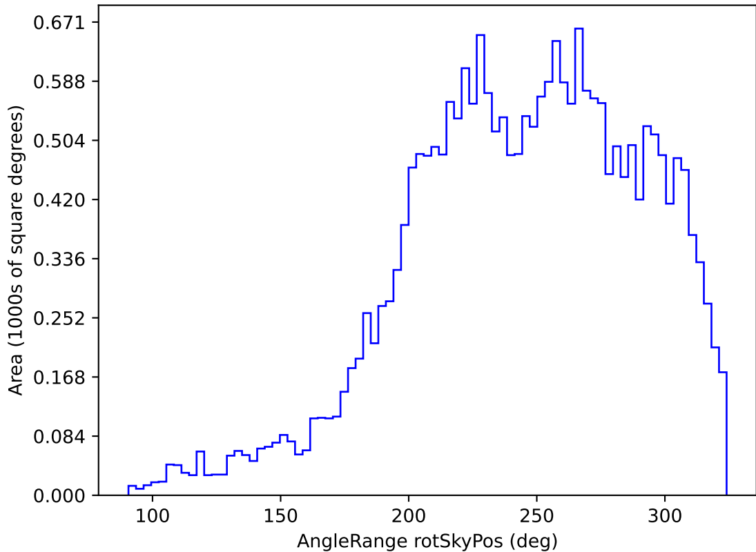
ddf_loaded_fl2_v3.4_10yrs All sky u band: AngleRange rotSkyPos
