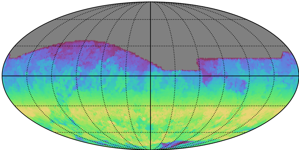
ddf_loaded_fl2_v3.4_10yrs All sky r band: AngleRange rotSkyPos
