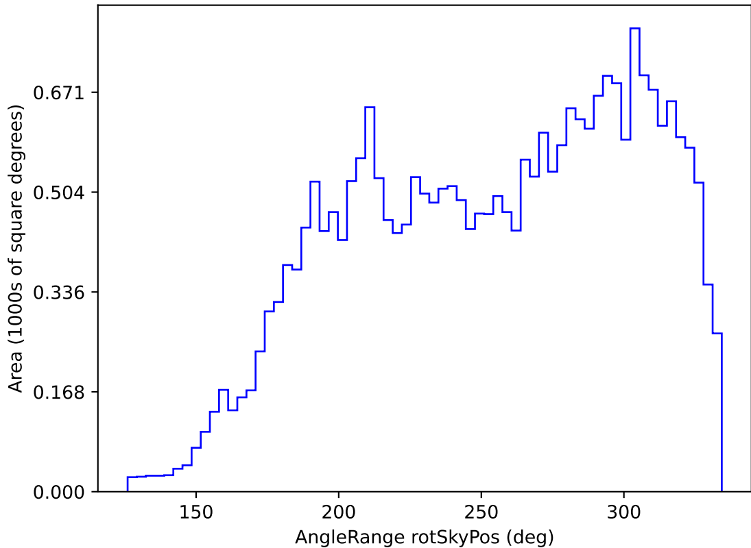
ddf_loaded_fl2_v3.4_10yrs All sky g band: AngleRange rotSkyPos
