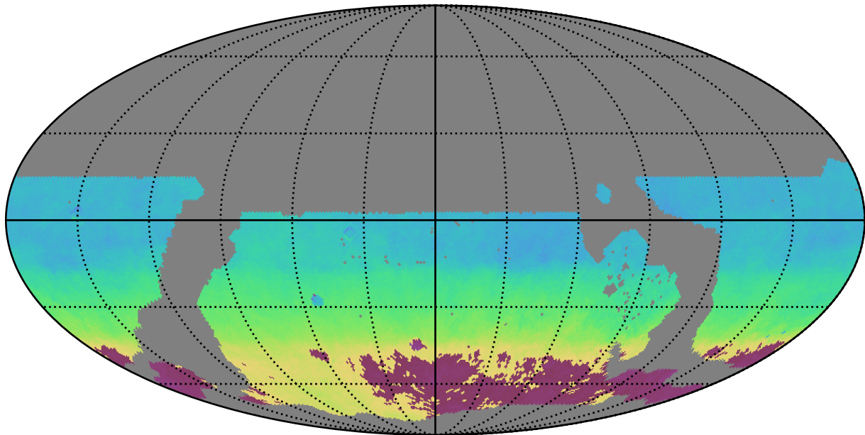
ddf_loaded_fl2_v3.4_10yrs WFD z band: AngleMean rotSkyPos
