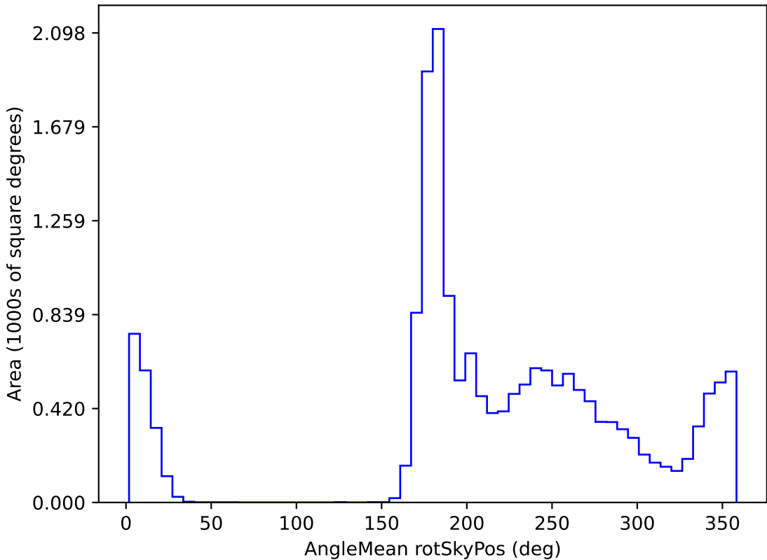
ddf_loaded_fl2_v3.4_10yrs WFD z band: AngleMean rotSkyPos
