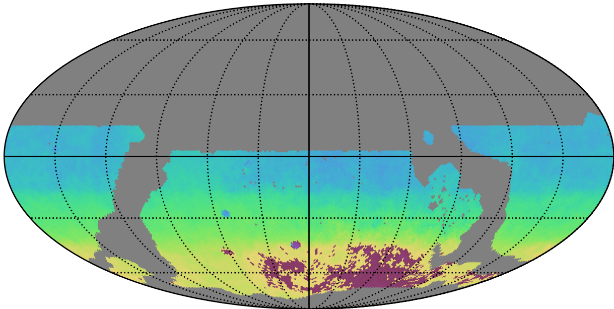
ddf_loaded_fl2_v3.4_10yrs WFD y band: AngleMean rotSkyPos
