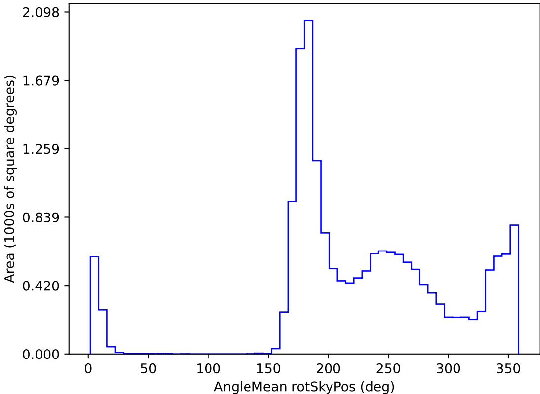
ddf_loaded_fl2_v3.4_10yrs WFD y band: AngleMean rotSkyPos
