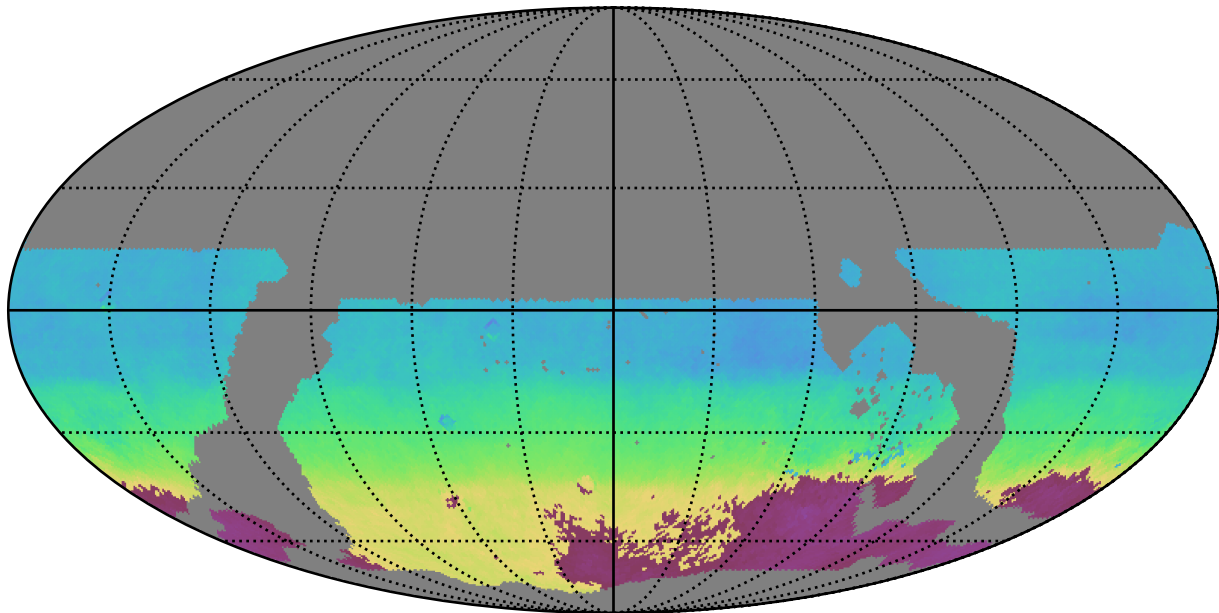
ddf_loaded_fl2_v3.4_10yrs WFD r band: AngleMean rotSkyPos
