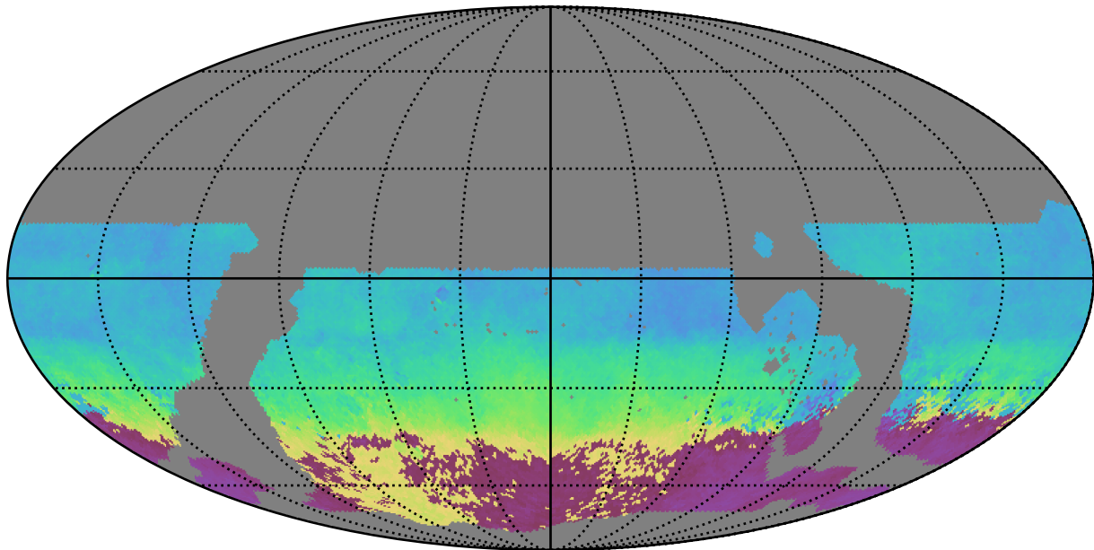
ddf_loaded_fl2_v3.4_10yrs WFD g band: AngleMean rotSkyPos
