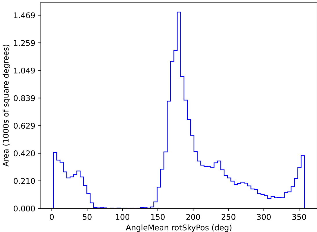
ddf_loaded_fl2_v3.4_10yrs WFD g band: AngleMean rotSkyPos
