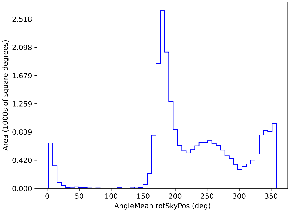
ddf_loaded_fl2_v3.4_10yrs All sky y band: AngleMean rotSkyPos
