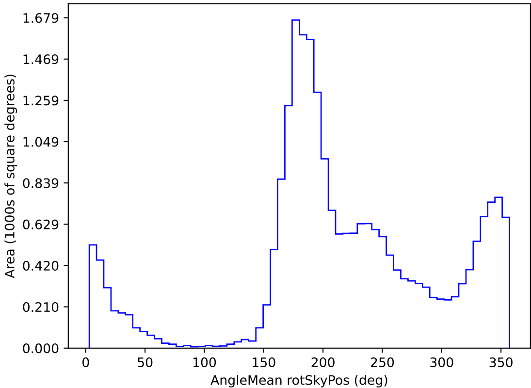
ddf_loaded_fl2_v3.4_10yrs All sky u band: AngleMean rotSkyPos
