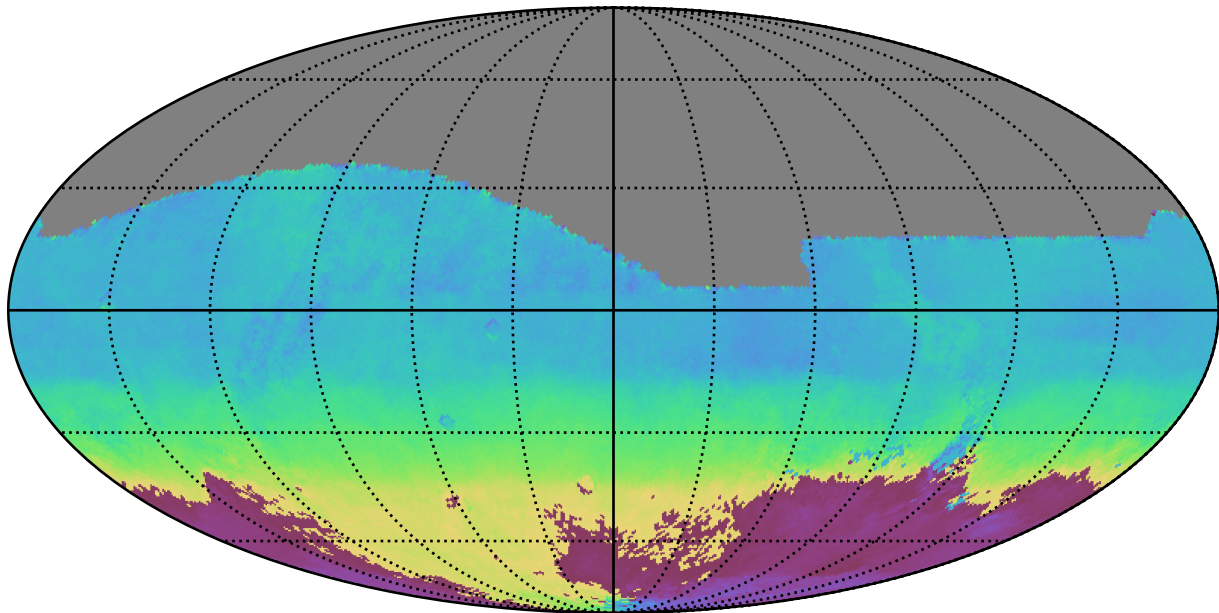
ddf_loaded_fl2_v3.4_10yrs All sky r band: AngleMean rotSkyPos
