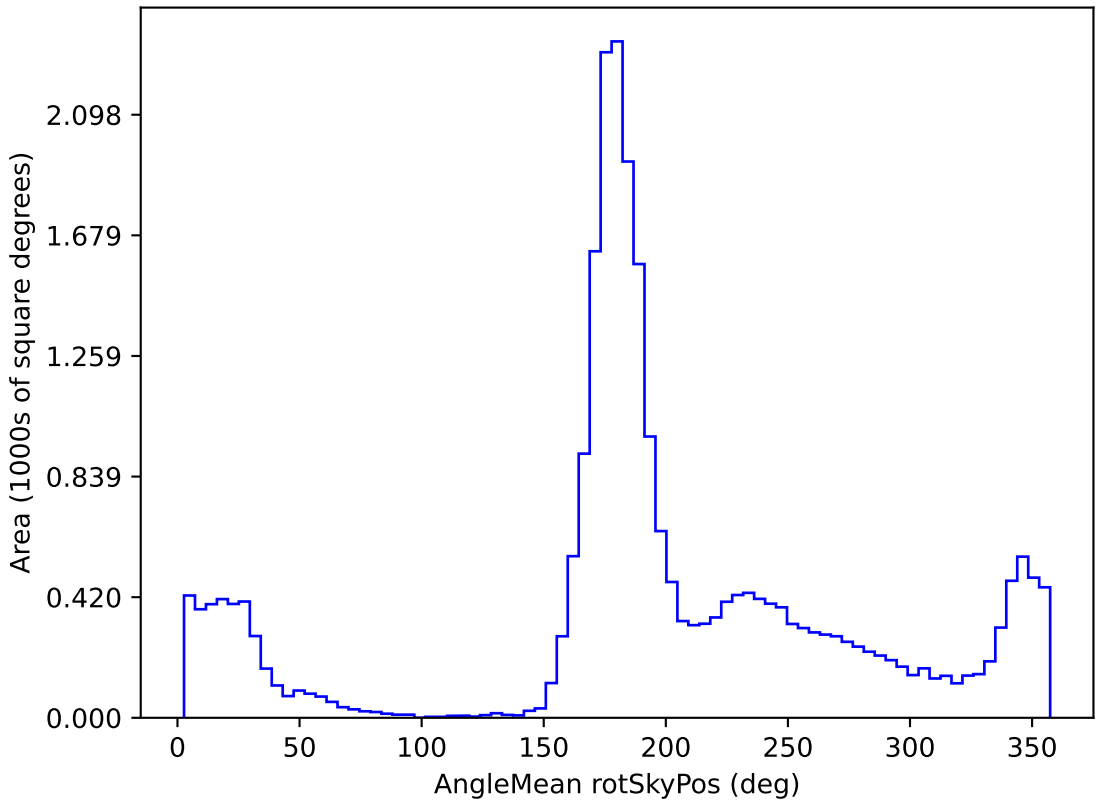
ddf_loaded_fl2_v3.4_10yrs All sky r band: AngleMean rotSkyPos
