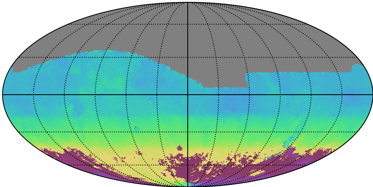
ddf_loaded_fl2_v3.4_10yrs All sky i band: AngleMean rotSkyPos
