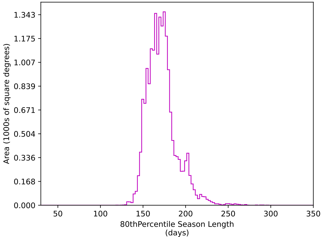
ddf_loaded_fl2_v3.4_10yrs WFD z band: 80thPercentile Season Length
