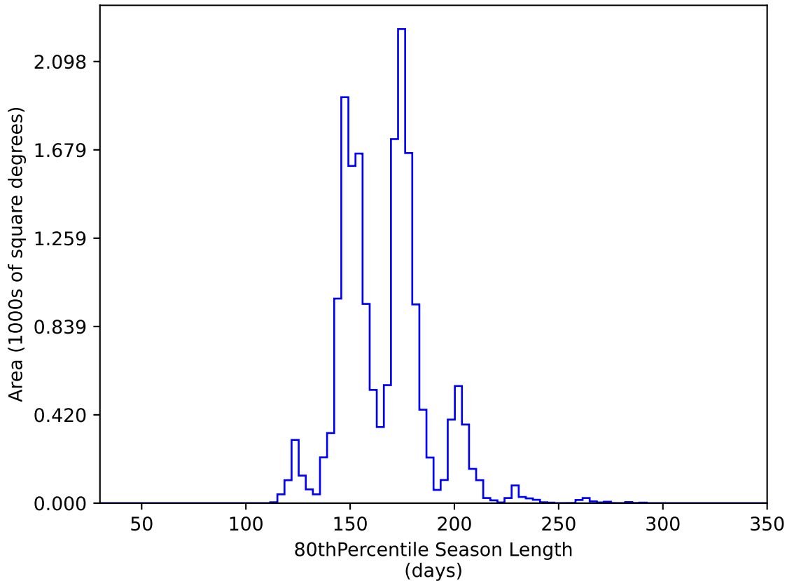
ddf_loaded_fl2_v3.4_10yrs WFD y band: 80thPercentile Season Length
