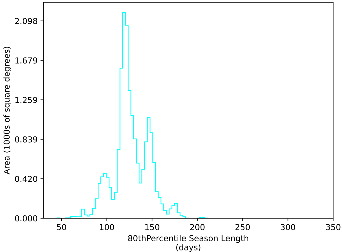
ddf_loaded_fl2_v3.4_10yrs WFD u band: 80thPercentile Season Length
