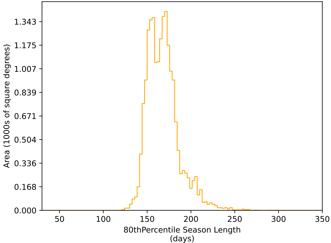
ddf_loaded_fl2_v3.4_10yrs WFD r band: 80thPercentile Season Length
