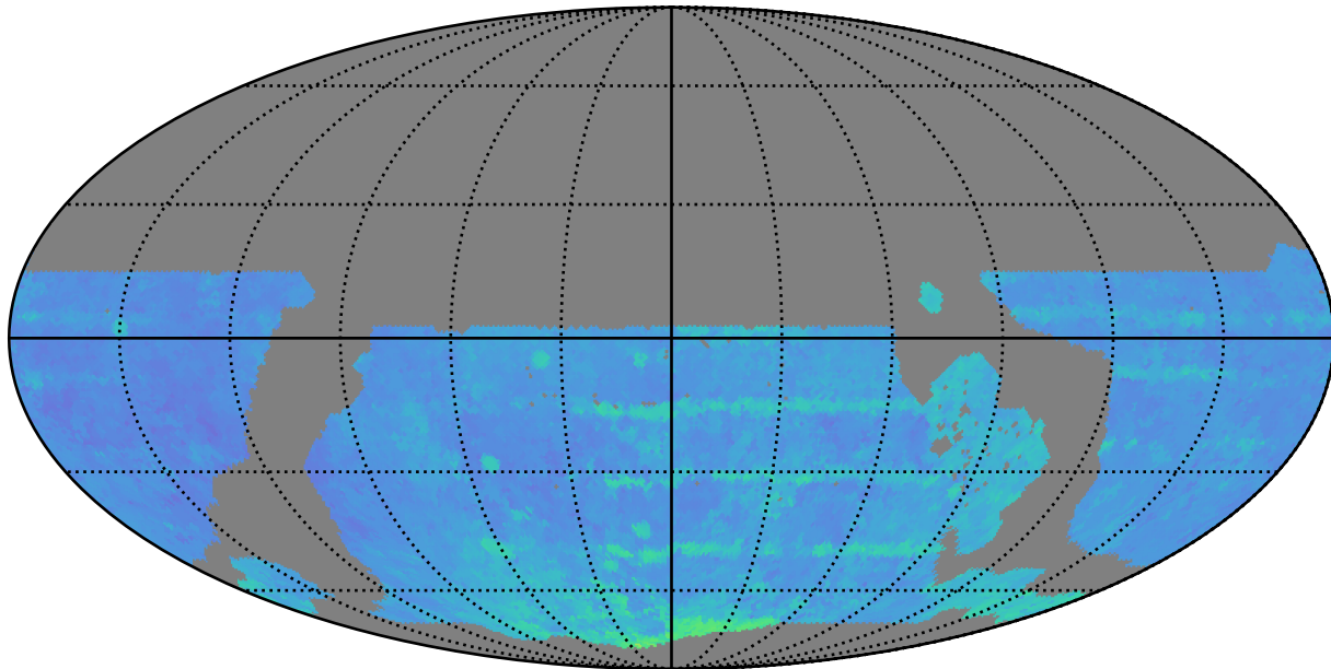
ddf_loaded_fl2_v3.4_10yrs WFD i band: 80thPercentile Season Length
