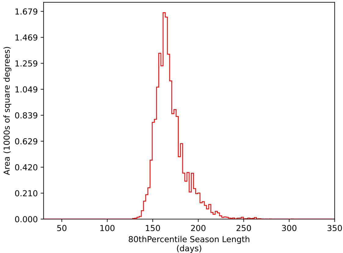
ddf_loaded_fl2_v3.4_10yrs WFD i band: 80thPercentile Season Length
