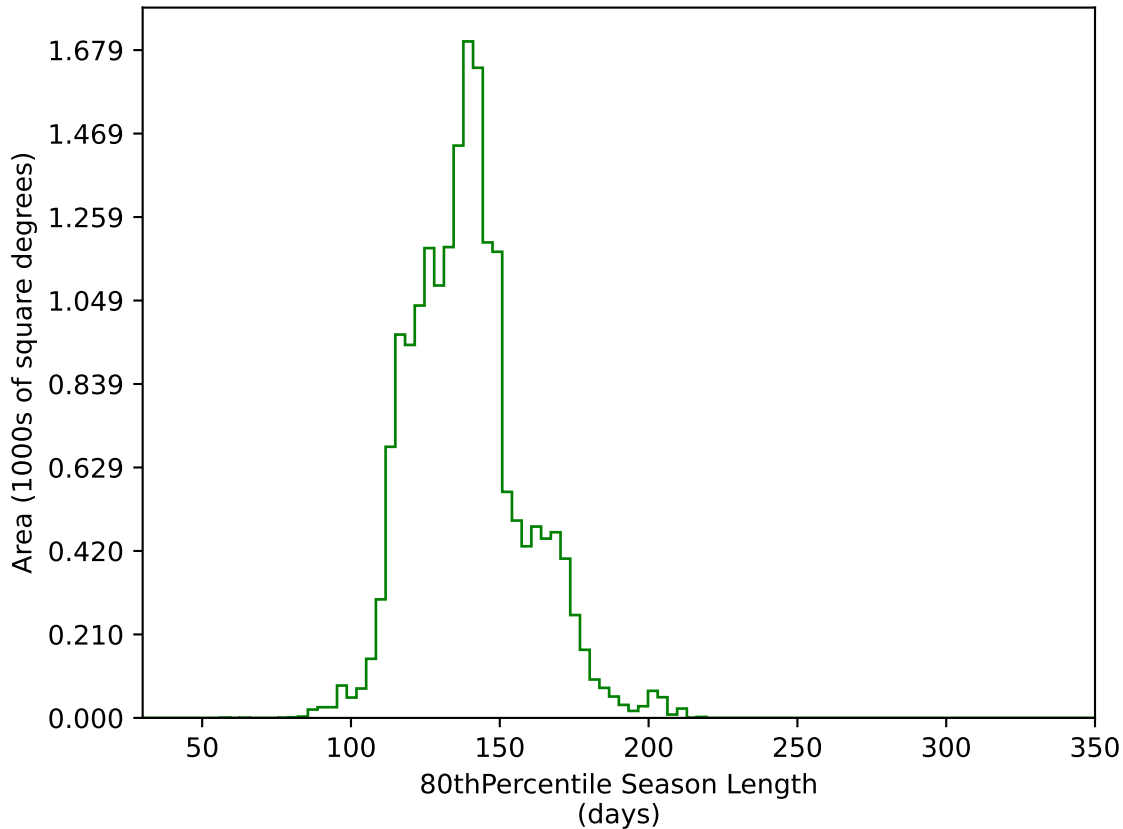
ddf_loaded_fl2_v3.4_10yrs WFD g band: 80thPercentile Season Length
