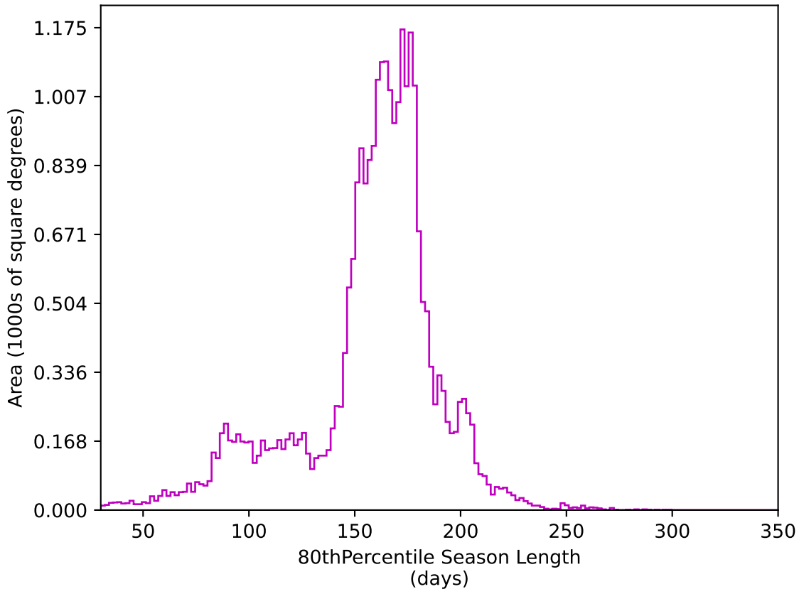
ddf_loaded_fl2_v3.4_10yrs All sky z band: 80thPercentile Season Length
