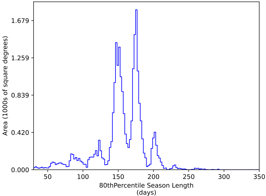
ddf_loaded_fl2_v3.4_10yrs All sky y band: 80thPercentile Season Length
