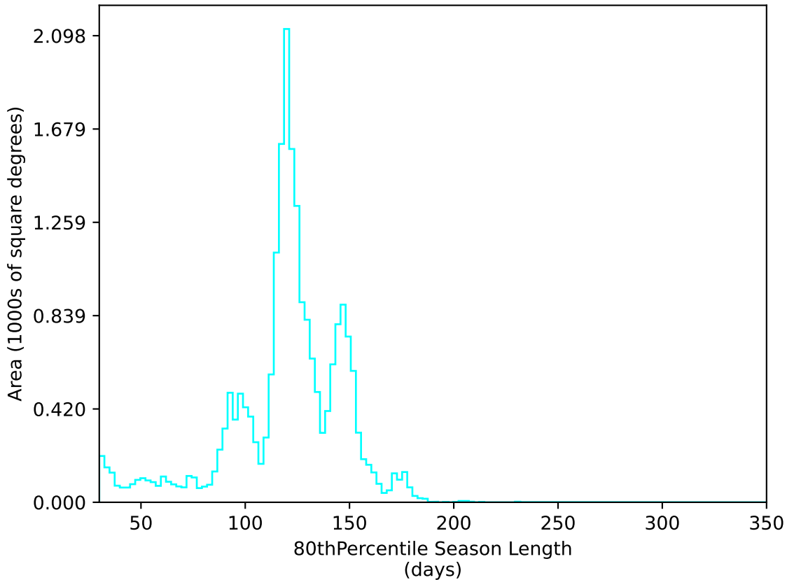
ddf_loaded_fl2_v3.4_10yrs All sky u band: 80thPercentile Season Length
