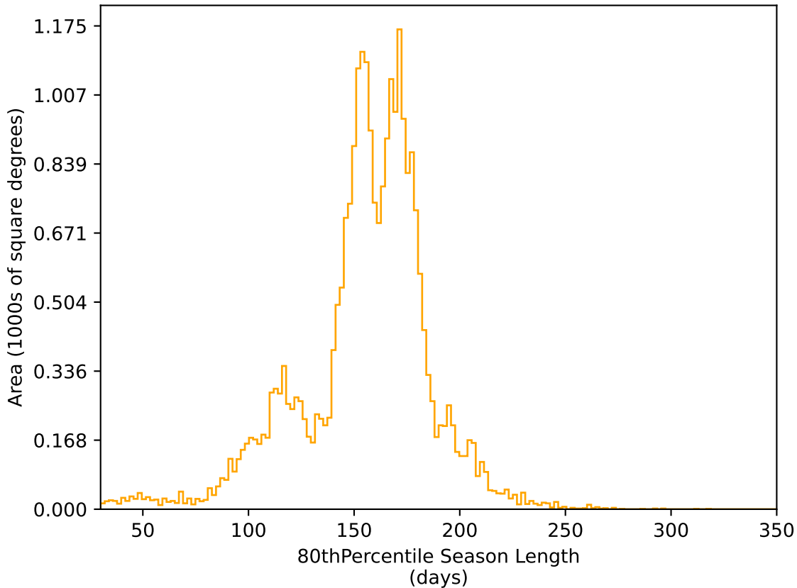
ddf_loaded_fl2_v3.4_10yrs All sky r band: 80thPercentile Season Length
