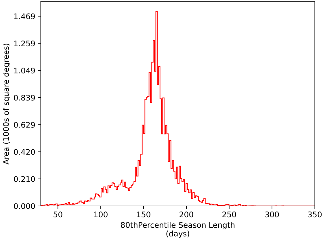
ddf_loaded_fl2_v3.4_10yrs All sky i band: 80thPercentile Season Length
