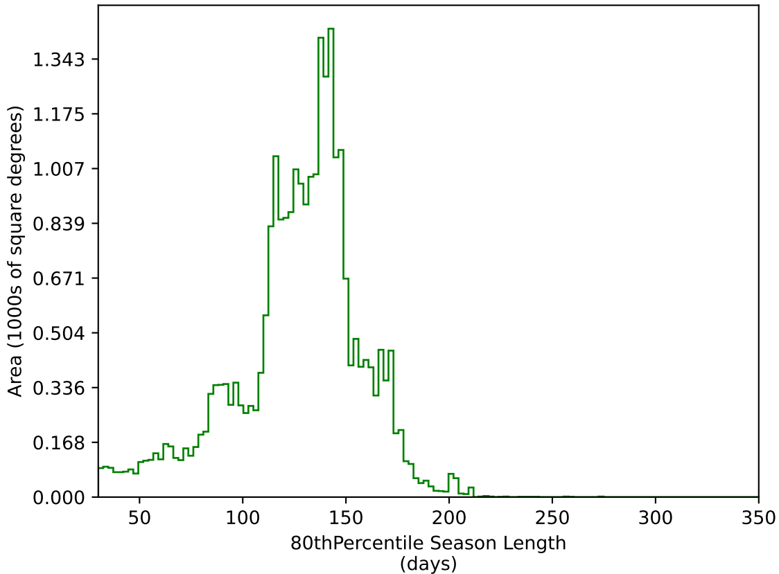
ddf_loaded_fl2_v3.4_10yrs All sky g band: 80thPercentile Season Length
