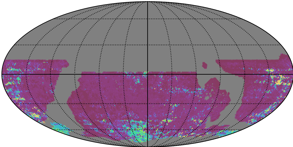
ddf_loaded_fl2_v3.4_10yrs WFD z band: 75th Percentile Intranight Timespan
