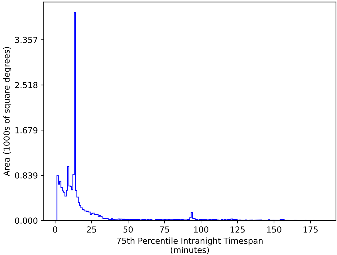
ddf_loaded_fl2_v3.4_10yrs WFD z band: 75th Percentile Intranight Timespan
