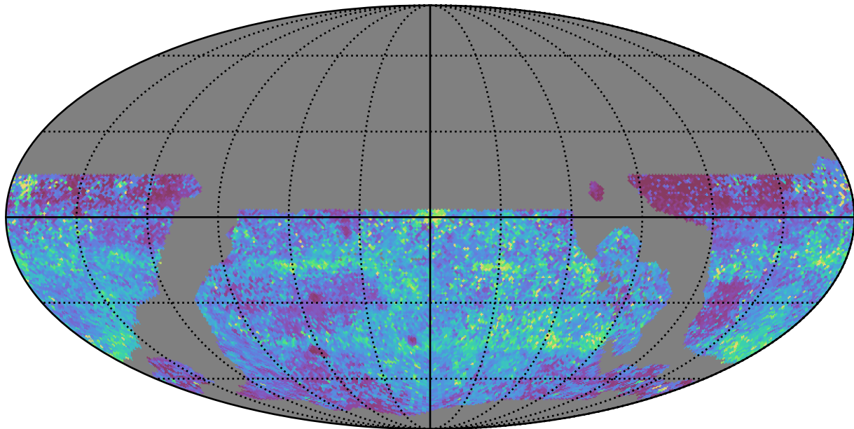
ddf_loaded_fl2_v3.4_10yrs WFD y band: 75th Percentile Intranight Timespan
