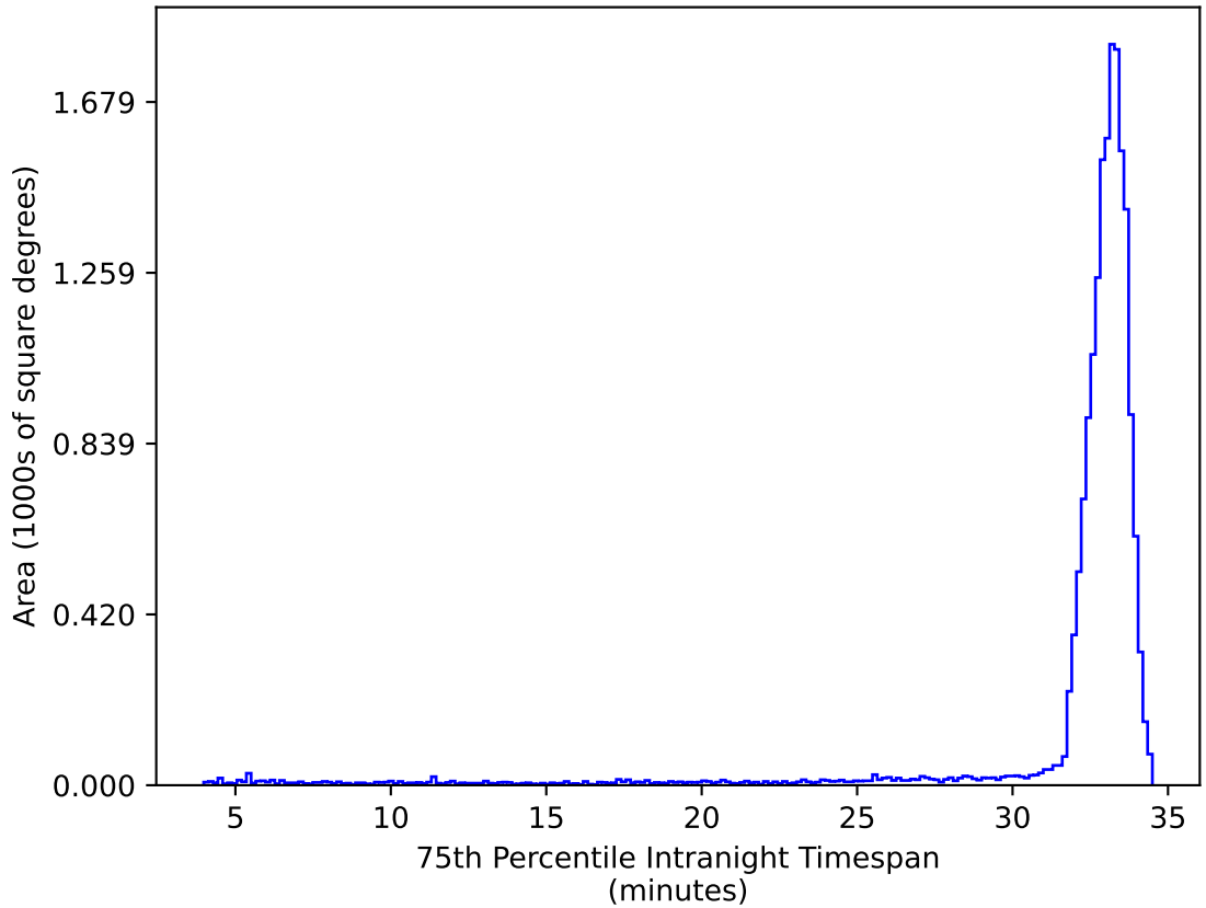
ddf_loaded_fl2_v3.4_10yrs WFD ug bands: 75th Percentile Intranight Timespan
