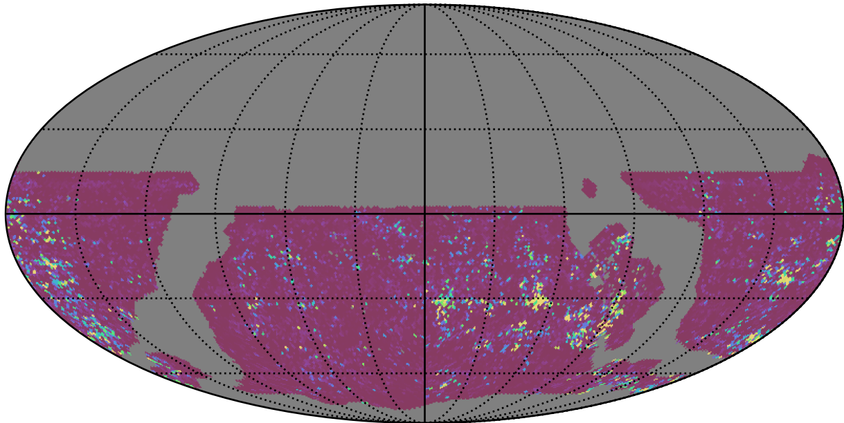
ddf_loaded_fl2_v3.4_10yrs WFD u band: 75th Percentile Intranight Timespan
