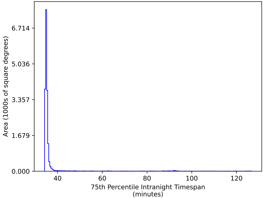
ddf_loaded_fl2_v3.4_10yrs WFD ri bands: 75th Percentile Intranight Timespan
