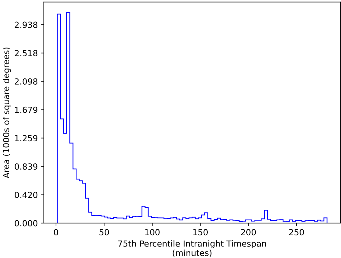
ddf_loaded_fl2_v3.4_10yrs WFD r band: 75th Percentile Intranight Timespan
