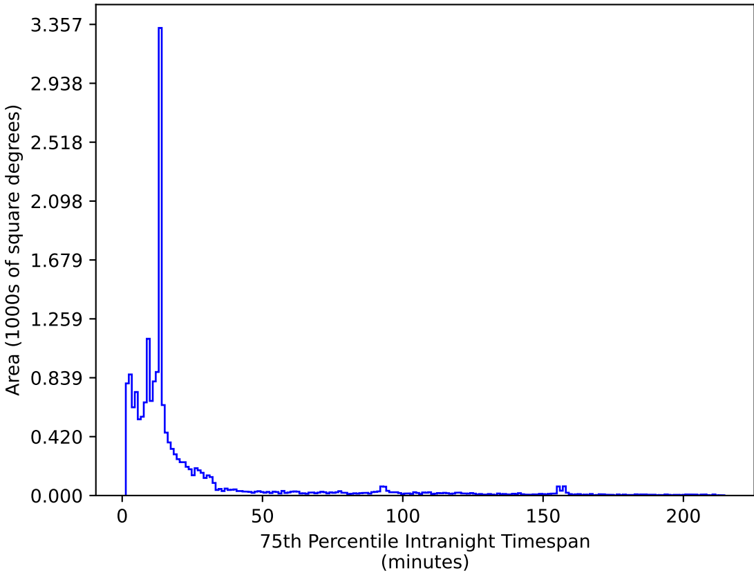
ddf_loaded_fl2_v3.4_10yrs WFD i band: 75th Percentile Intranight Timespan
