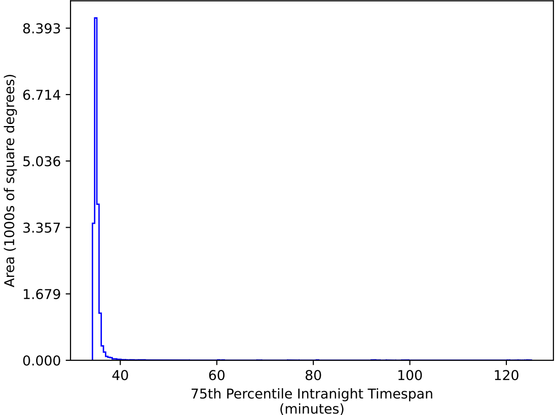
ddf_loaded_fl2_v3.4_10yrs WFD gr bands: 75th Percentile Intranight Timespan
