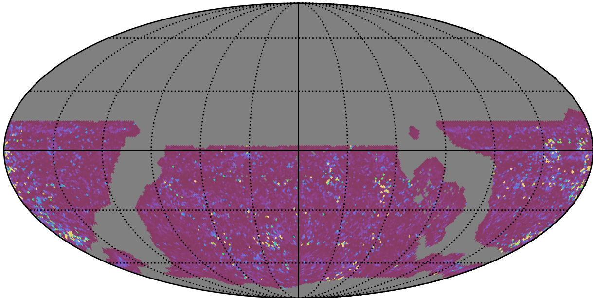
ddf_loaded_fl2_v3.4_10yrs WFD g band: 75th Percentile Intranight Timespan
