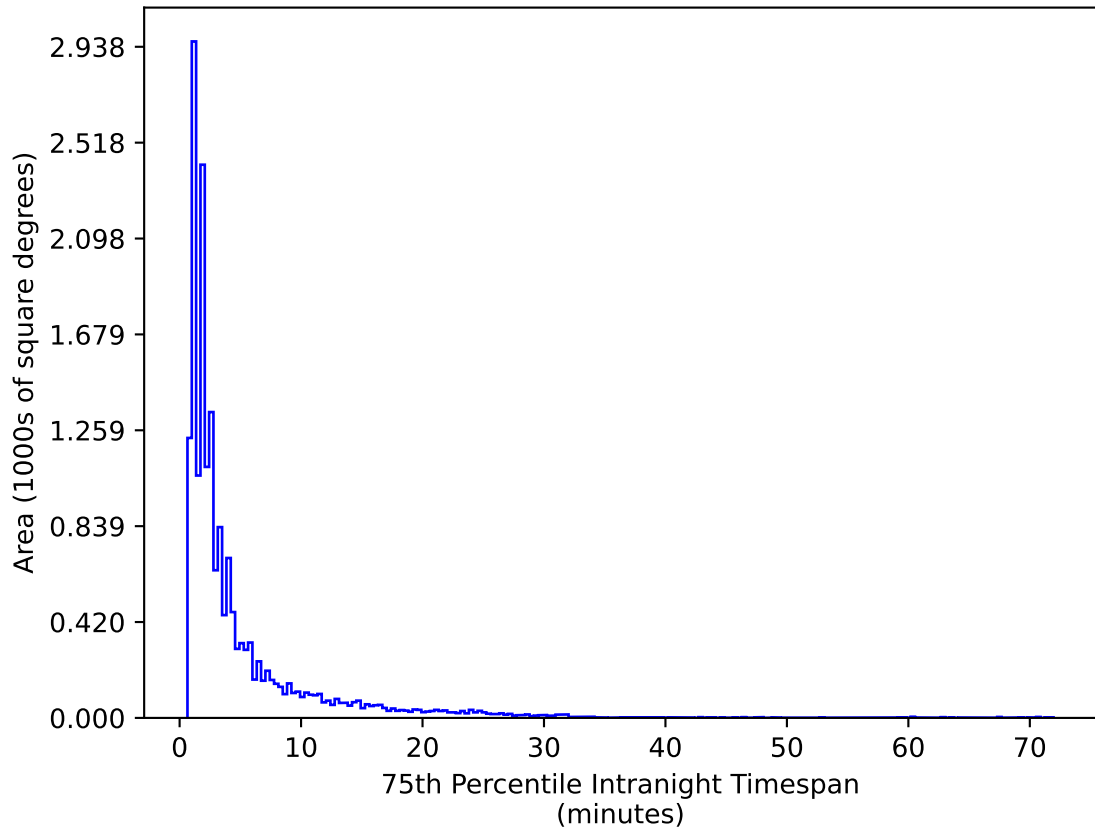
ddf_loaded_fl2_v3.4_10yrs WFD g band: 75th Percentile Intranight Timespan
