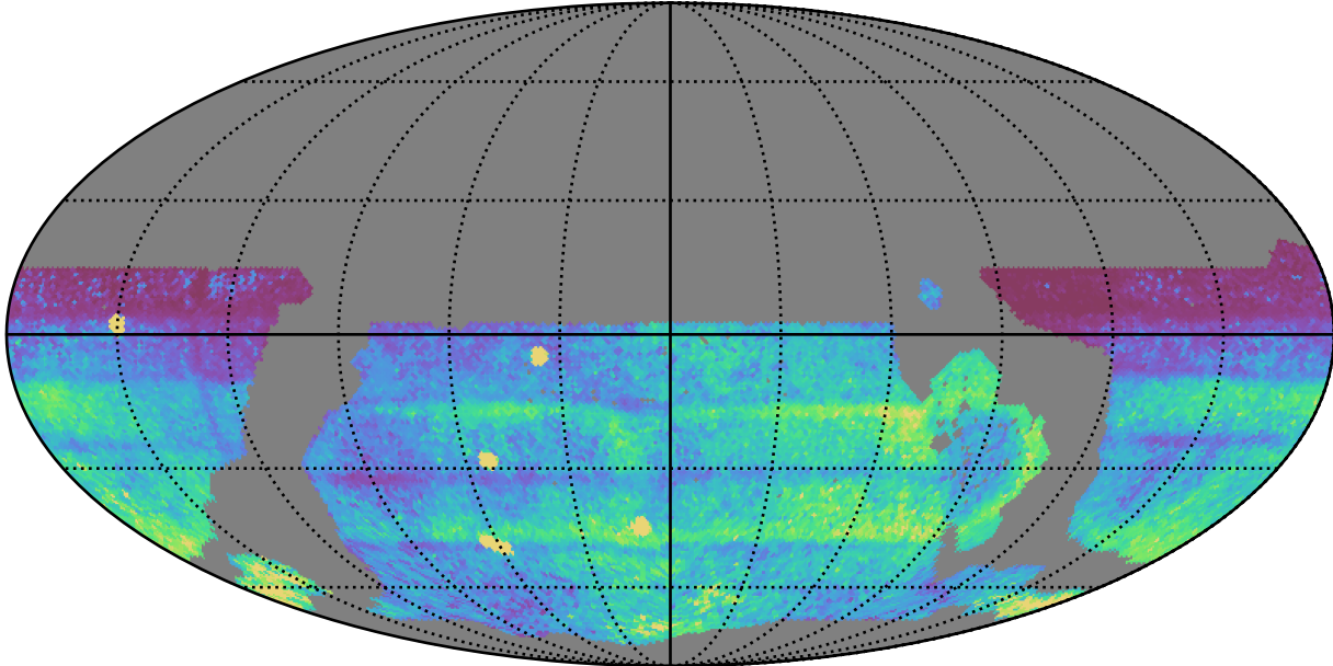
ddf_loaded_fl2_v3.4_10yrs WFD all bands: 75th Percentile Intranight Timespan
