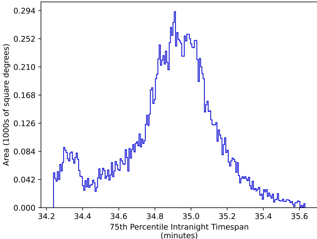
ddf_loaded_fl2_v3.4_10yrs WFD all bands: 75th Percentile Intranight Timespan
