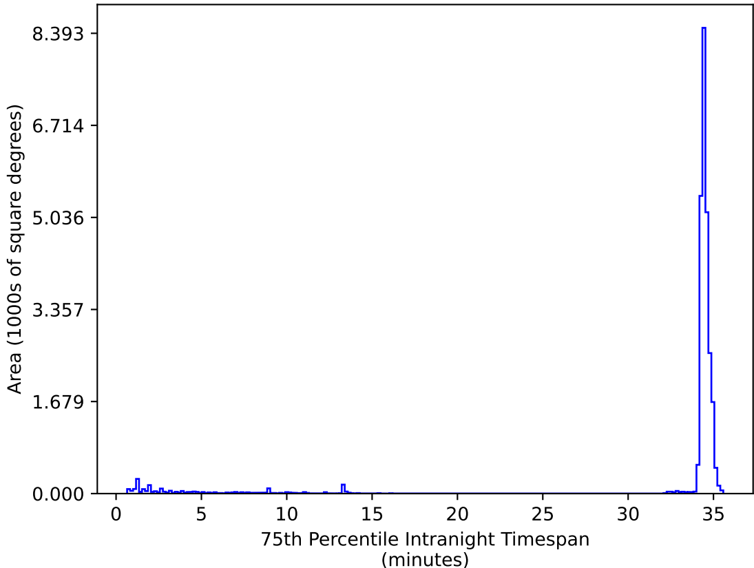
ddf_loaded_fl2_v3.4_10yrs All sky zy bands: 75th Percentile Intranight Timespan
