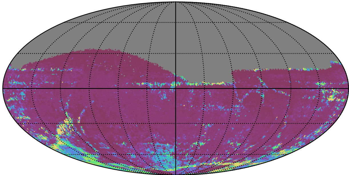
ddf_loaded_fl2_v3.4_10yrs All sky z band: 75th Percentile Intranight Timespan
