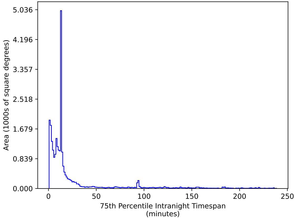
ddf_loaded_fl2_v3.4_10yrs All sky z band: 75th Percentile Intranight Timespan
