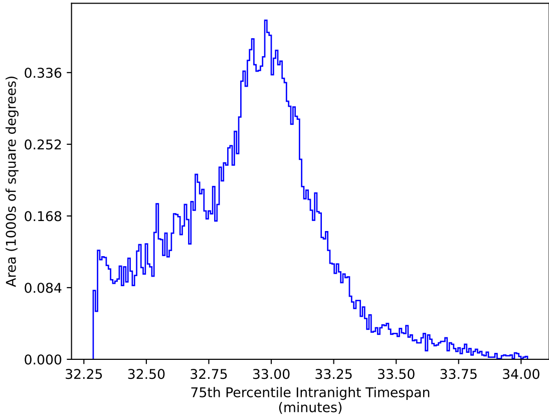
ddf_loaded_fl2_v3.4_10yrs All sky y band: 75th Percentile Intranight Timespan
