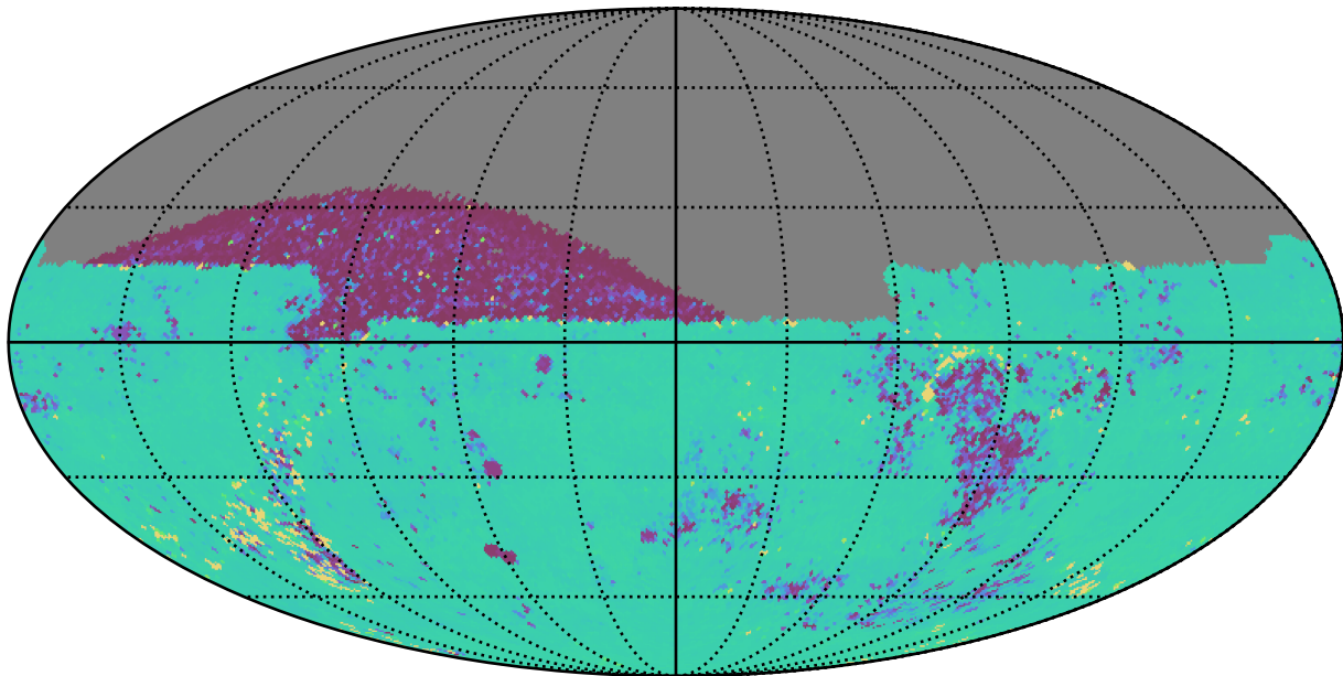
ddf_loaded_fl2_v3.4_10yrs All sky ug bands: 75th Percentile Intranight Timespan
