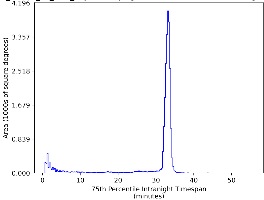
ddf_loaded_fl2_v3.4_10yrs All sky ug bands: 75th Percentile Intranight Timespan
